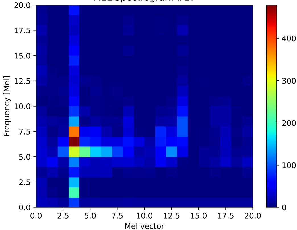
MEL Spectrogram #17
